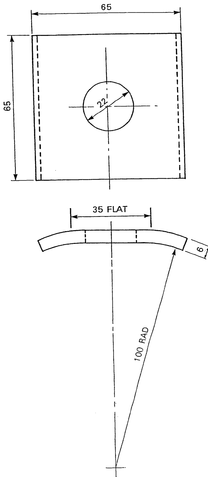
Fig. 3 Washer square (curved) (ESI Drawing 439605)
